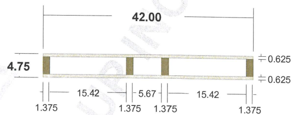
End View
